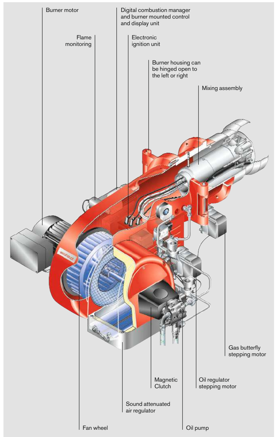
WM-GL30 version ZM-R
