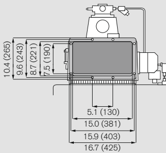
Ducted air intake bottom
