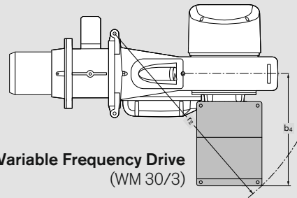
Burner mounted oil pump unit (WM 30/3)
