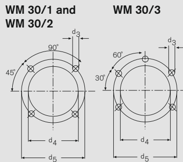
Boiler plate mounting dimensions
