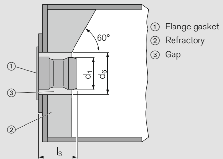
Mounting to heat exchanger
